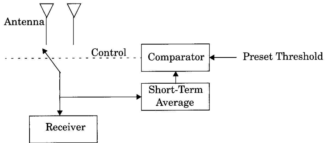
Figure 7.13 Basic form of scanning diversity.
